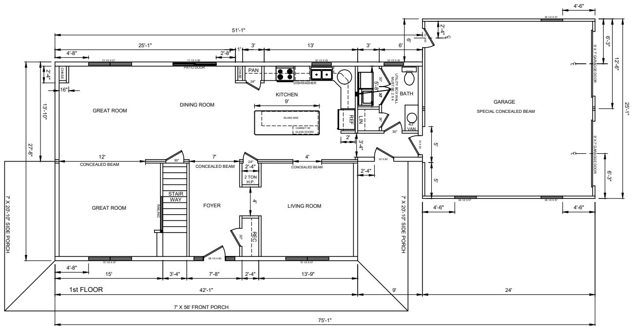
PLAN #31 2,478 SQ. FT.
