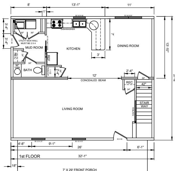
PLAN #28 1,792 SQ. FT.
