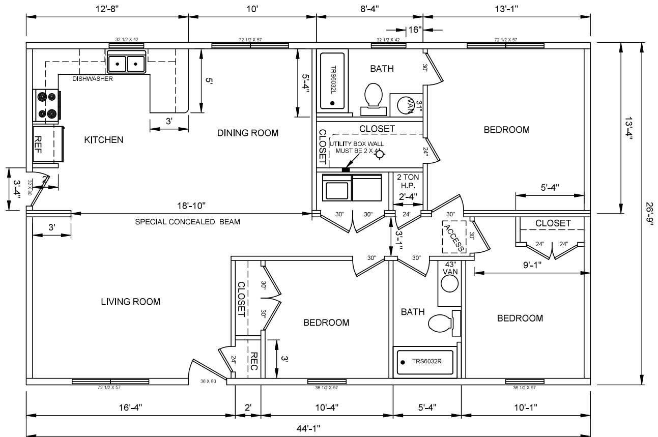
FLOOR PLAN #3 1,177 SQ. FT.
