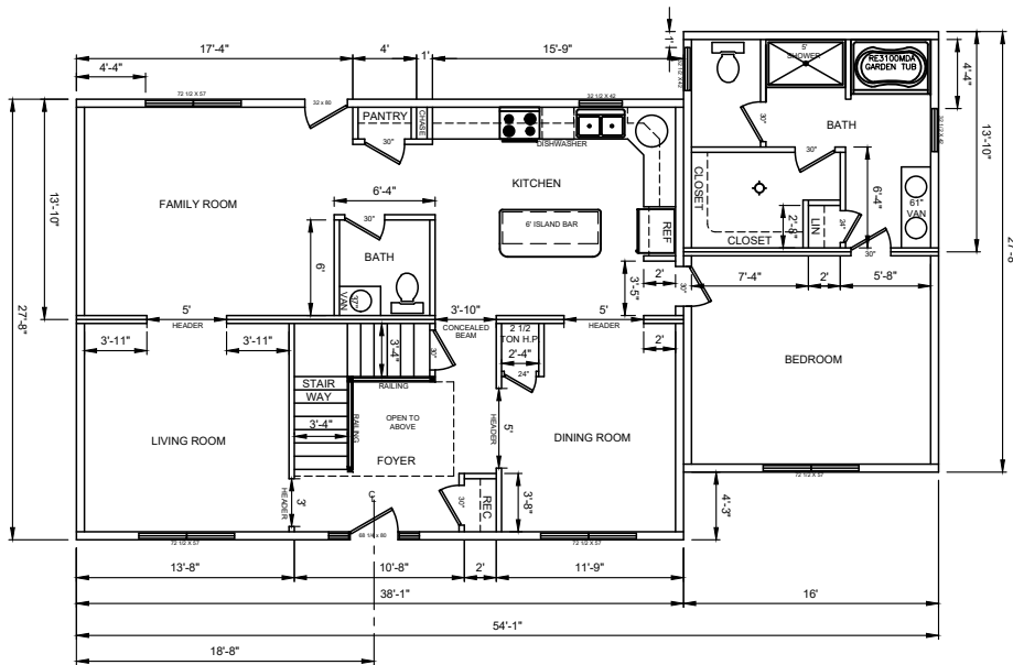
FLOOR PLAN #32 2,576 SQ. FT.
