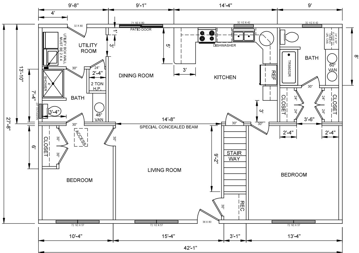
FLOOR PLAN #2 1,176 SQ.FT.
