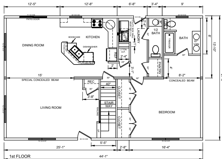
PLAN #25 1,980 SQ. FT.
