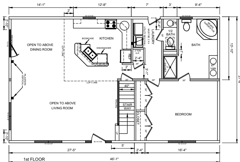
PLAN #19 1,917 SQ. FT.
